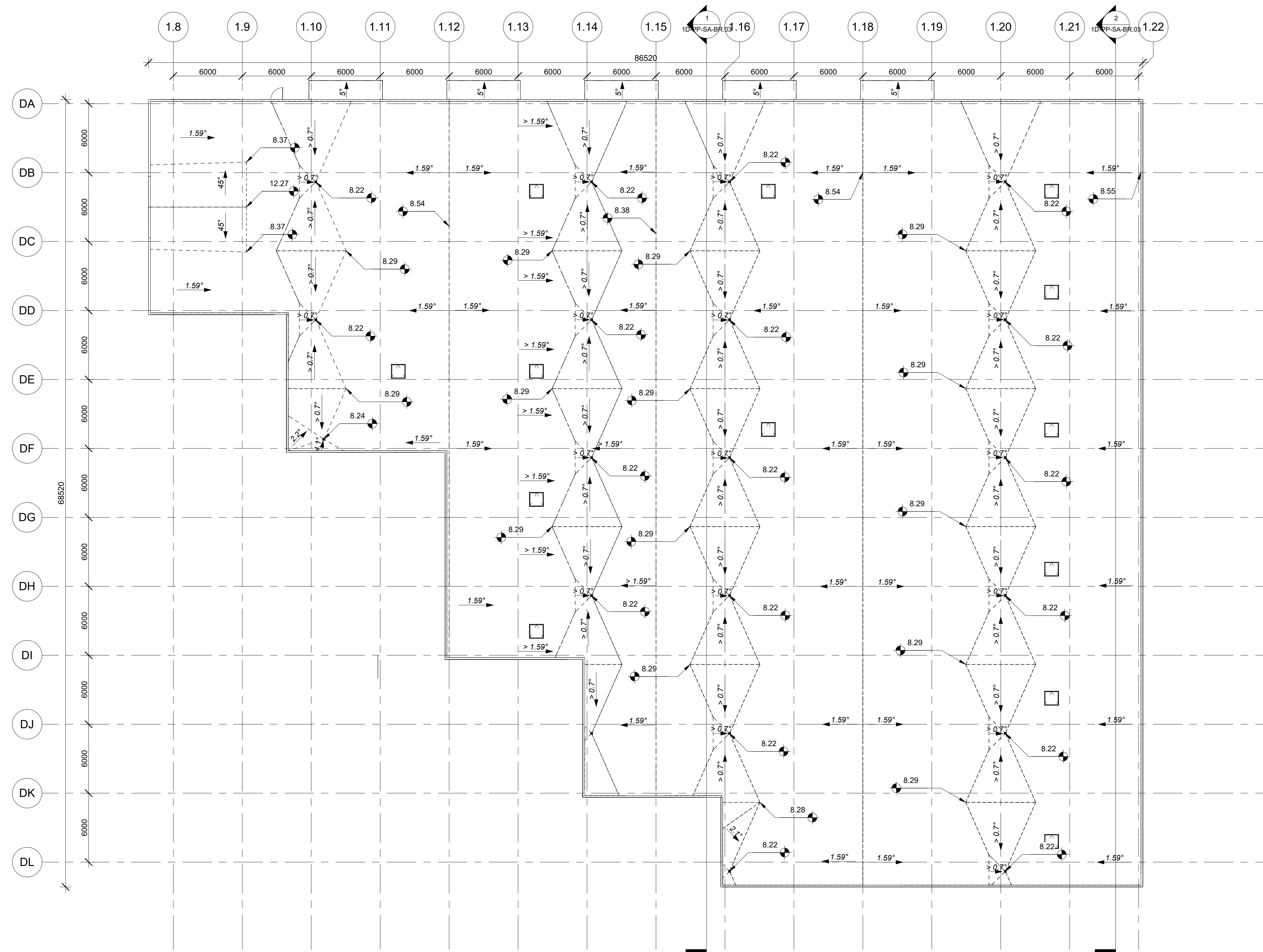
1 Pastatas 1D - Stogo planas 1 : 200
