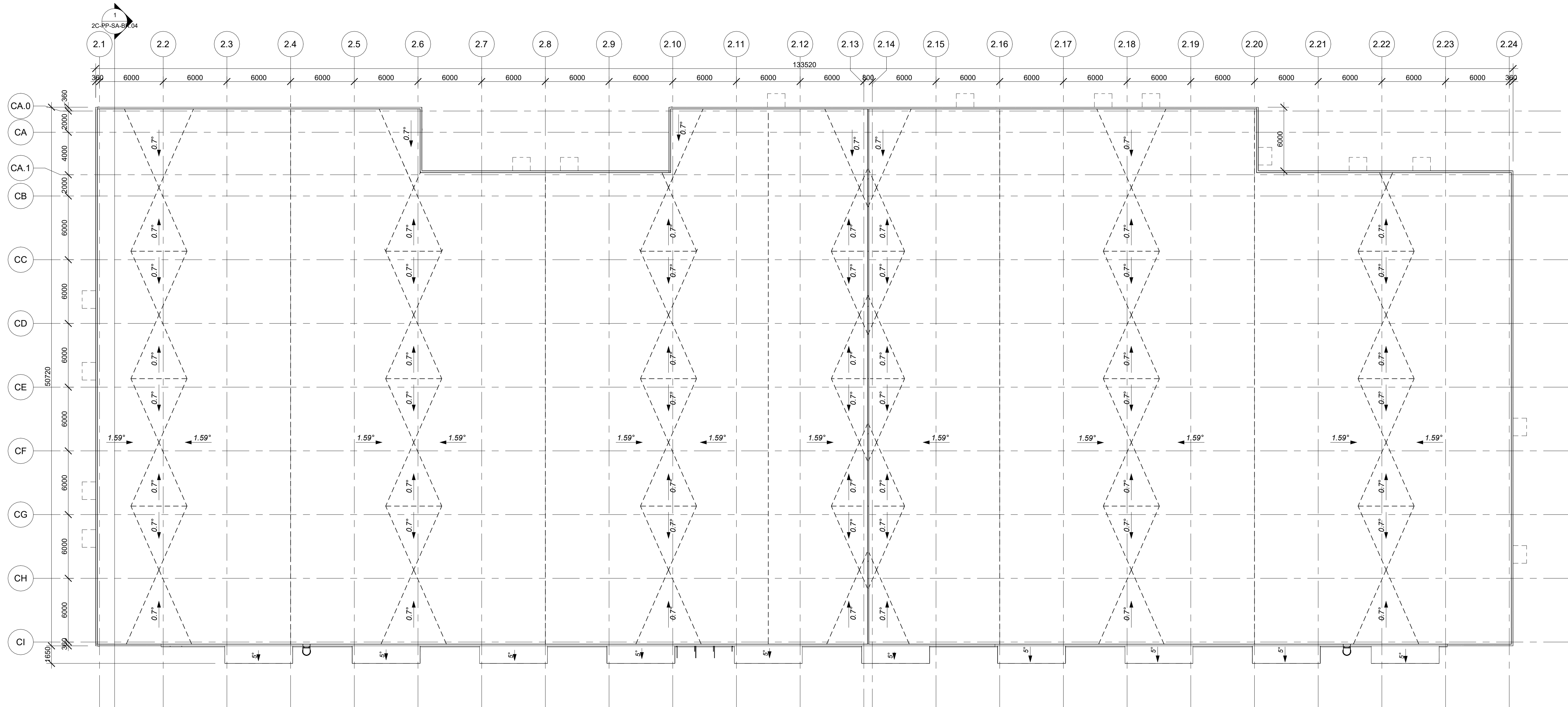
1 Pastatas 2C - Stogo planas 1:200
