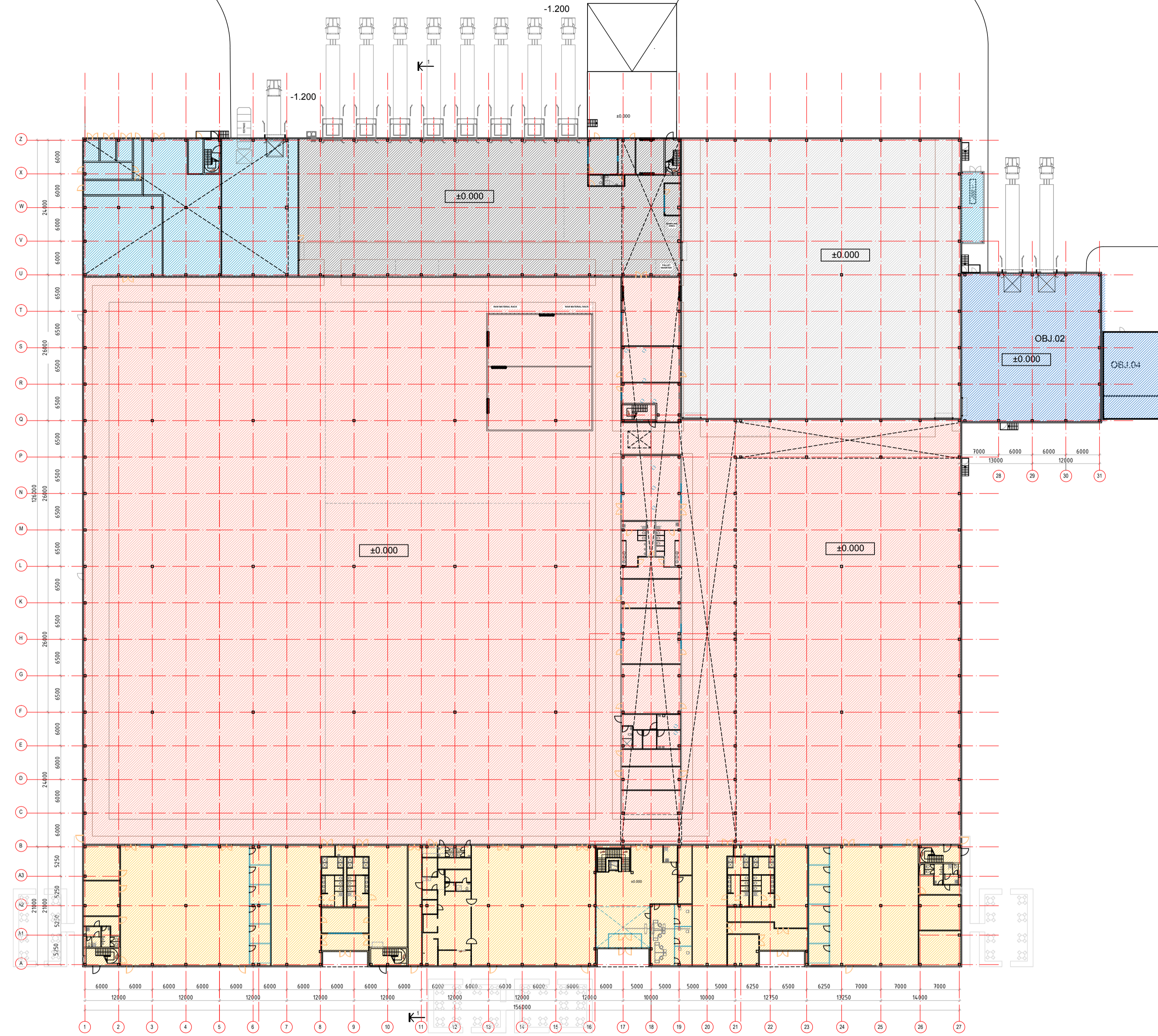
PLANAS/ PLAN ALT.+0.000 M 1:500
