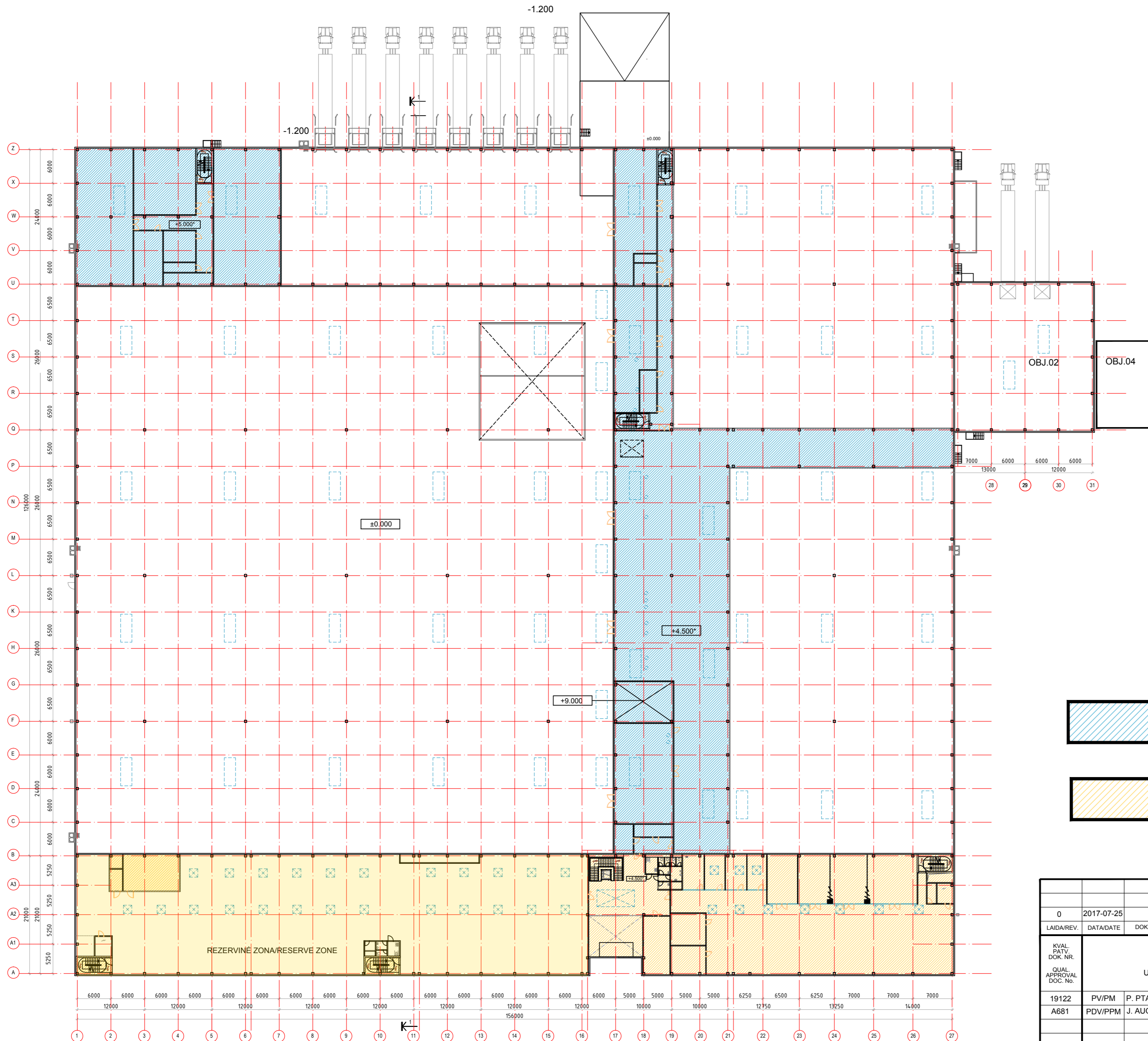
PLANAS/ PLAN ALT. +4.50* M 1:500
