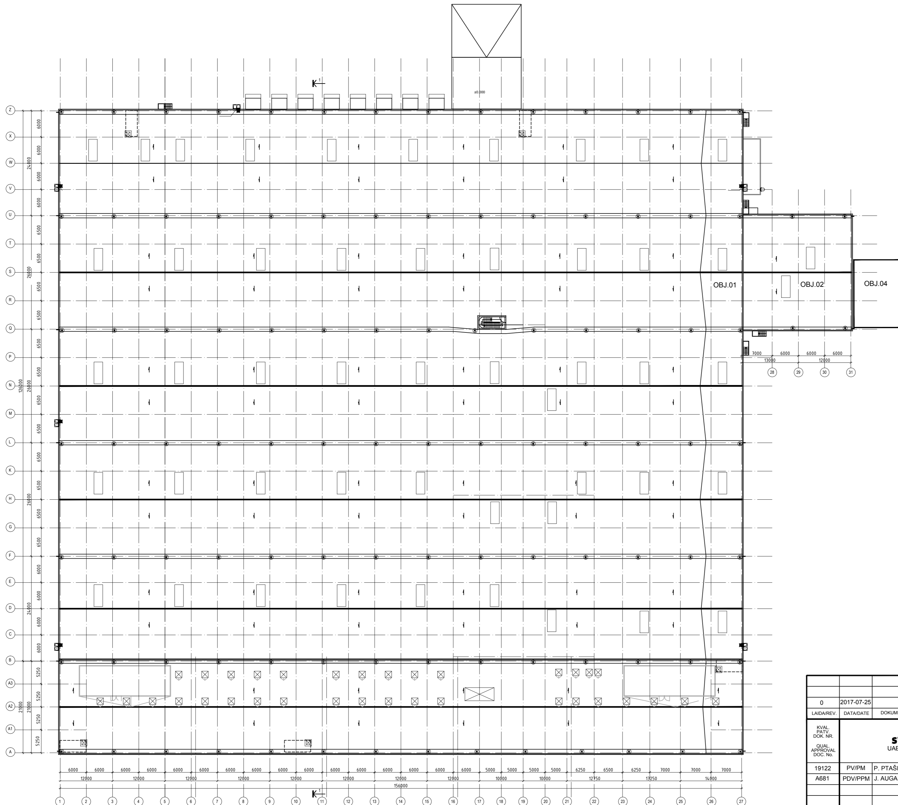
STOGO PLANO SCHEMA / ROOF PLAN SHCEME
